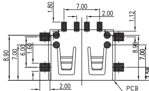
FRONT EDGE OF CONNECTOR PCB LAYOUT
