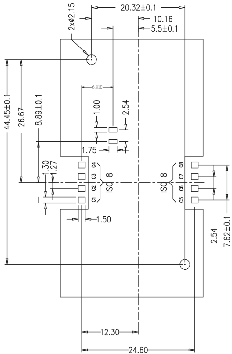
RECOMMENDED P.C.B. LAYOUT
